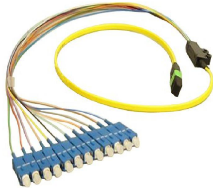
Ribbon cable+Fanout
