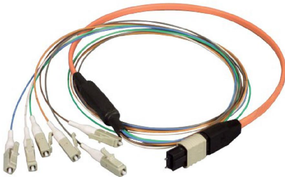
Round cable+Fanout
