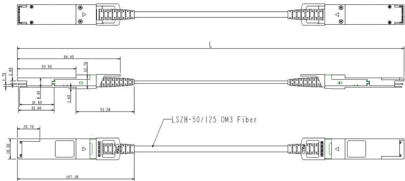
Figure9. Mechanical Specifications
