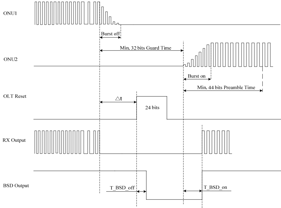
Figure 2 Reset Timing
