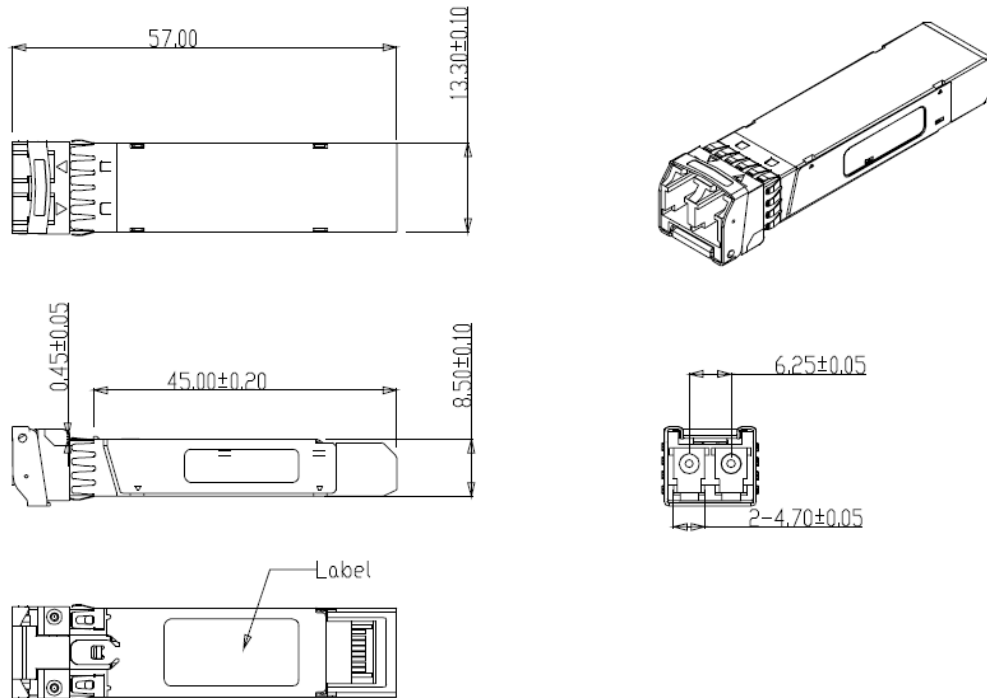
Figure5. Mechanical Specifications
