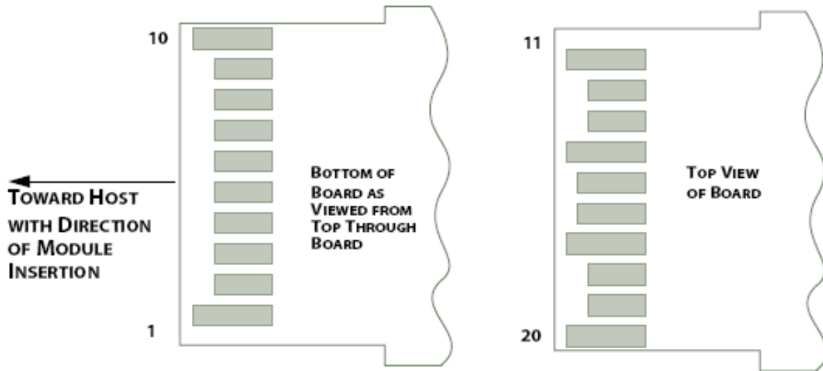
Figure 2: Module Contact Assignment
