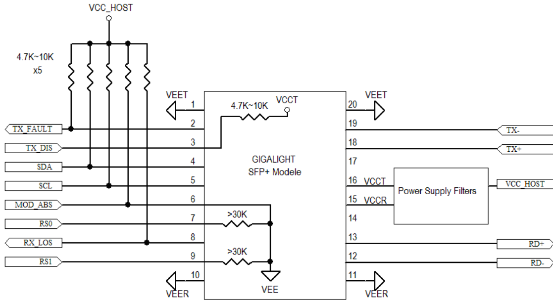
Figure4. Host-Module Interface
