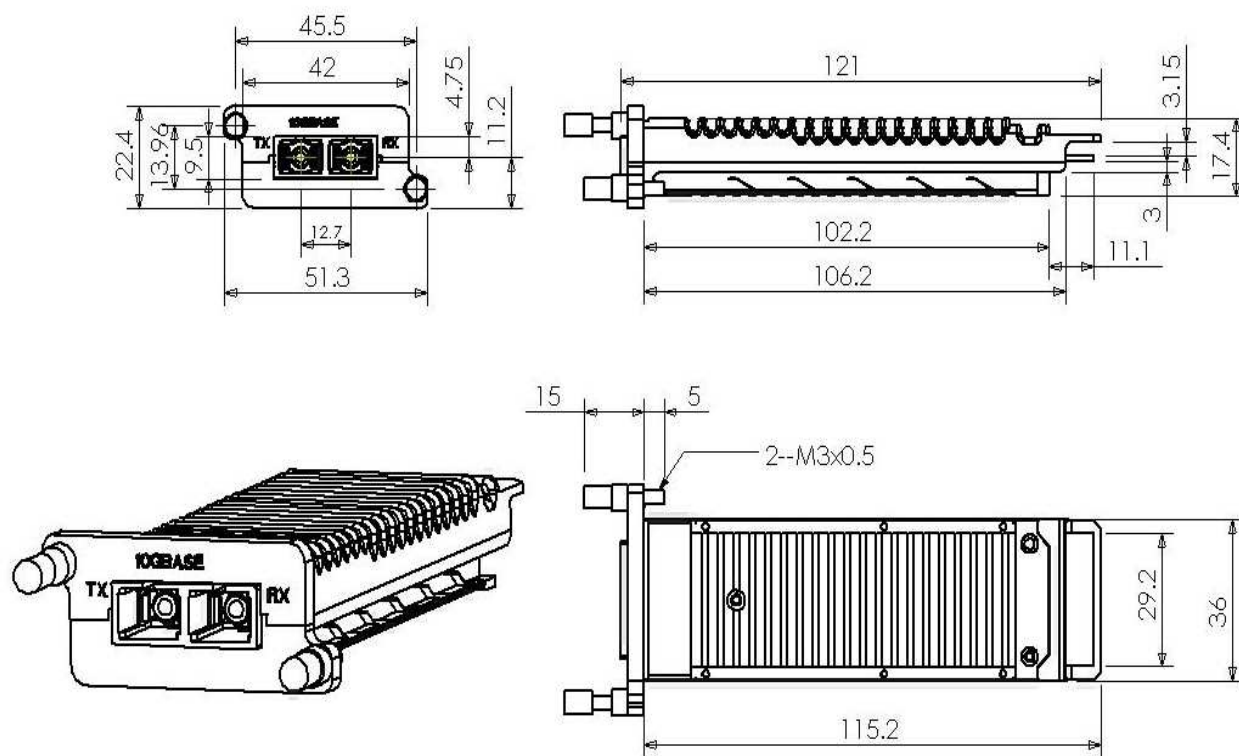
Figure 1 Mechanical dimensions
