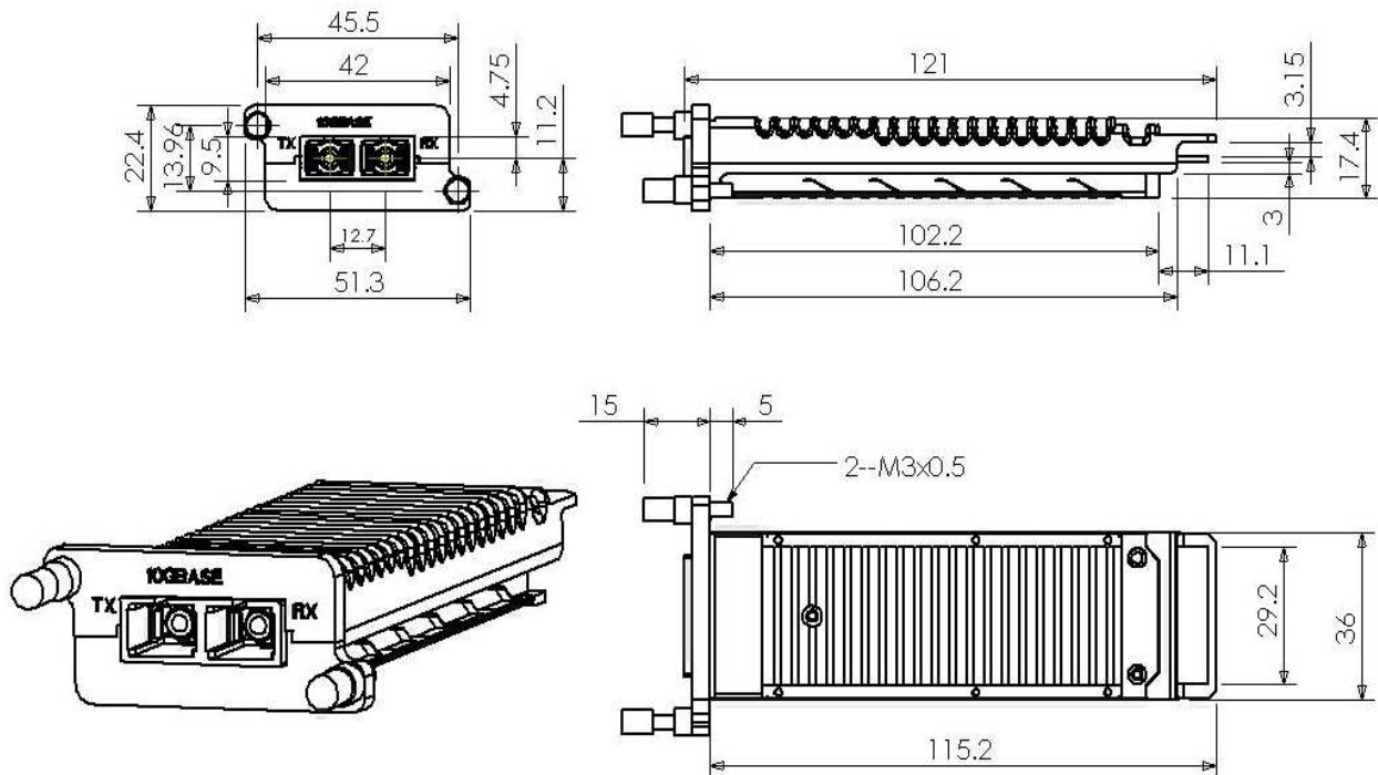
Figure 1 Mechanical dimensions
