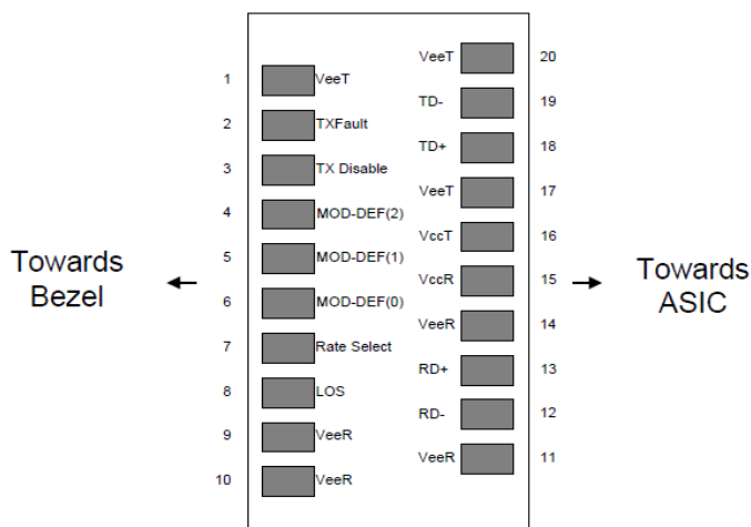
Figure 2: Pin-out of Connector Block on Host Board
